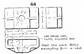
Figs. 1413-1415. Side-spring Yoke.
